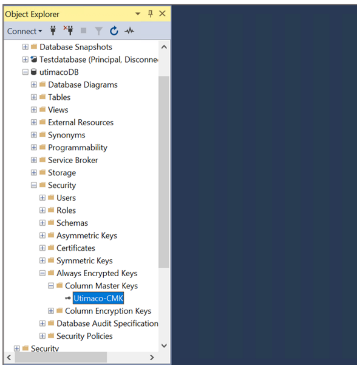
Figure 10 : New Column Master Key
