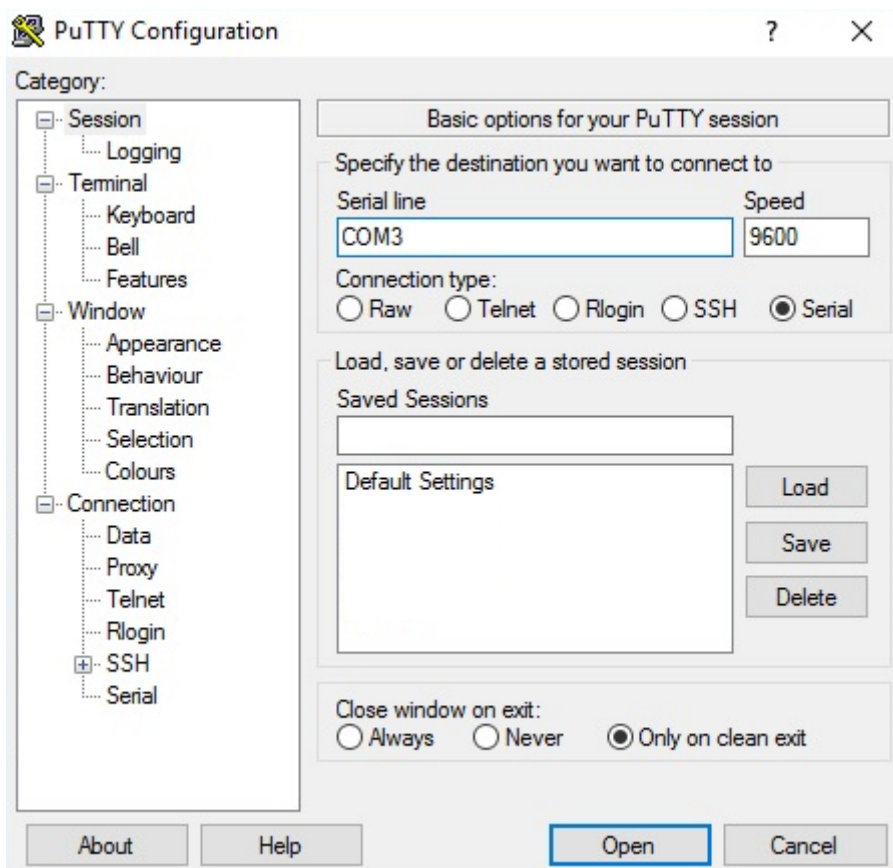
Figure 36 : Putty Configuration
