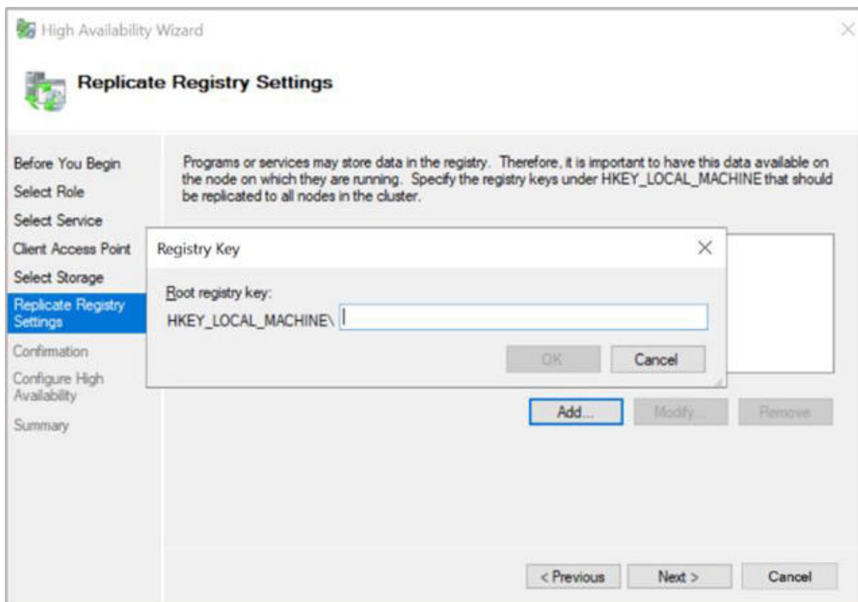
Figure 84 : "Replicate Registry Settings" Window
