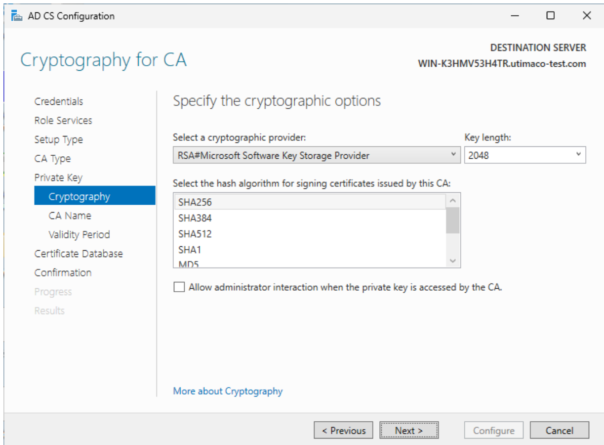
Figure 57 : "Cryptography for CA" Window
