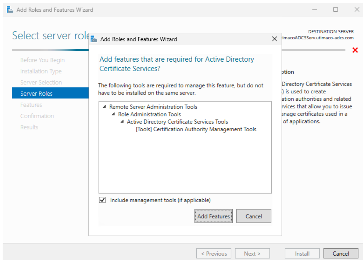
Figure 2 : "Add Roles and Features" Window
