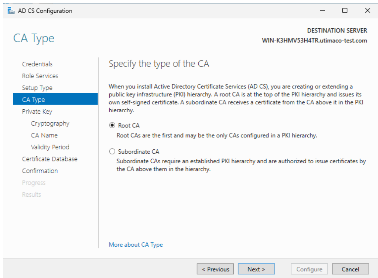
Figure 55 : "CA Type" Window
