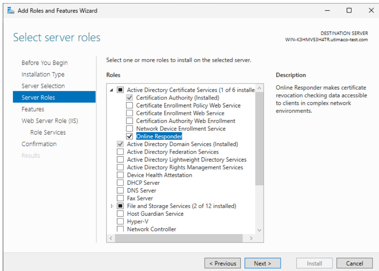
Figure 101 : "Select Server Roles" Window
