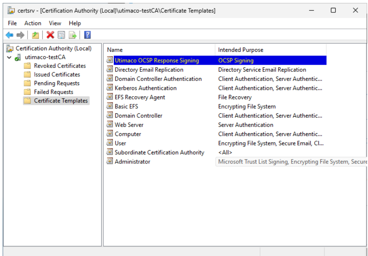
Figure 91 : "Certificate Authority" Window
