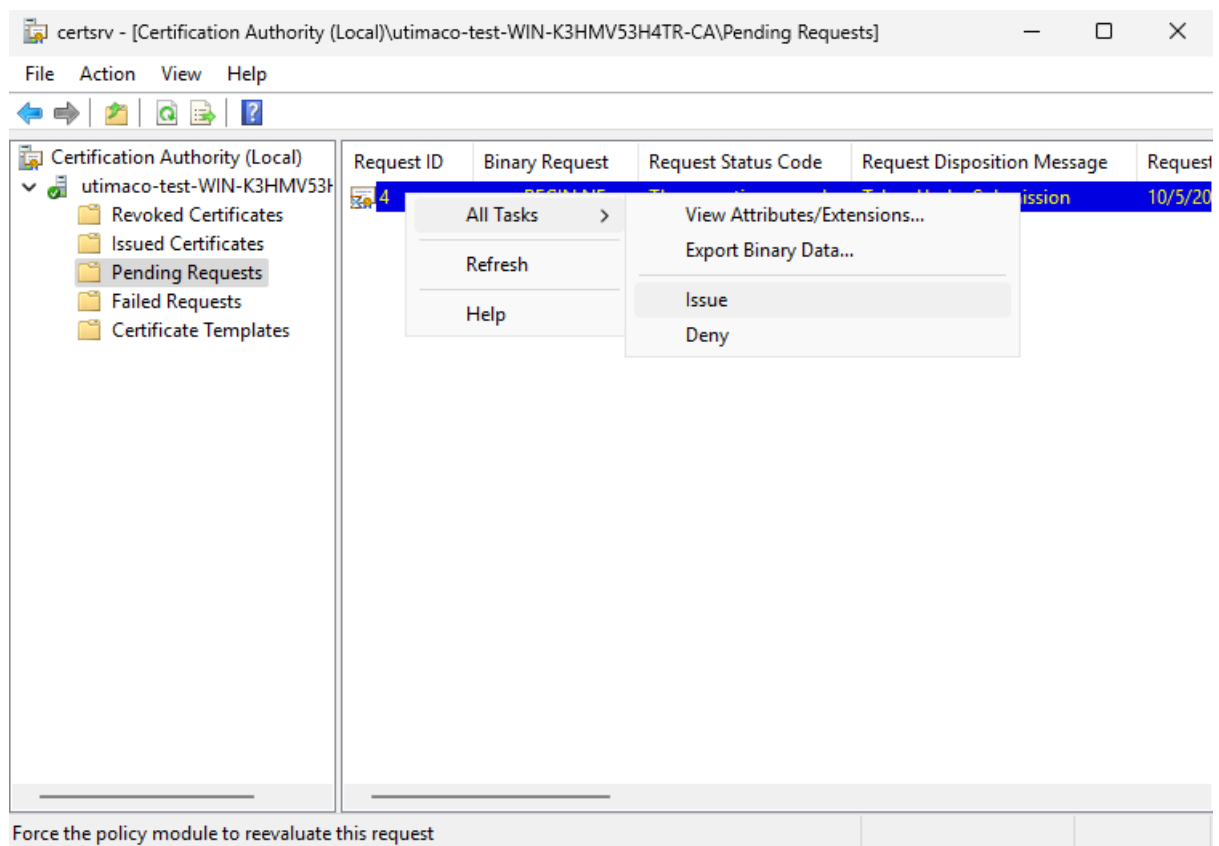
Figure 27 : "Certificate Authority" Window
